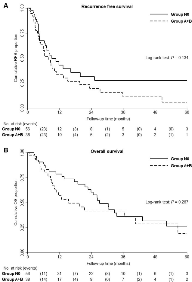
Supplementary Fig. 5. Kaplan-Meier survival curves of patients in groups N0 ( n = 56 ) and A + B ( n = 38 ). (A) Recurrence-free survival (RFS) for patients in groups N0 and A + B ( P = 0.134 ). (B) Overall survival (OS) for patients in groups N0 and A + B ( P = 0.267 ).
