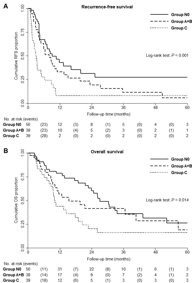
Supplementary Fig. 4. Kaplan-Meier survival curves of patients in groups N0 (n = 56), A + B (n = 38), and C (n = 39). (A) Recurrence-free survival (RFS) for patients in groups N0, A + B, and C ( P < 0.001 ). (B) Overall survival (OS) for patients in groups N0, A + B, and C ( P = 0.014 ).
