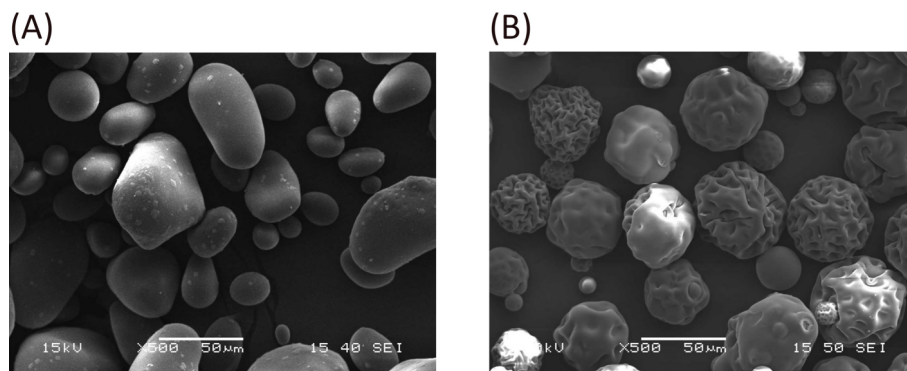
Supplementary Fig. 1. Scanning electron microscopic images for comparison of particle surface of (A) Oozfix (Theracion Biomedical, Seongnam, Korea) and (B) Arista AH (Bard, Murray Hill, NJ, USA).
