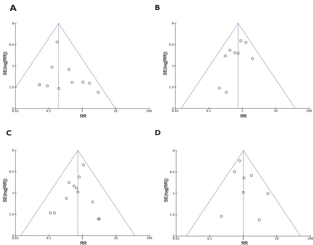
Supplementary Fig. 3. Funnel plots of risk ratios (RRs) and mean differences of perioperative and pathological outcomes. (A) Conversion rate, (B) circumferential resection margin involvement, (C) major complication (Clavien-Dindo classification III–V), and (D) incompleteness of mesorectum. SE, standard error.
