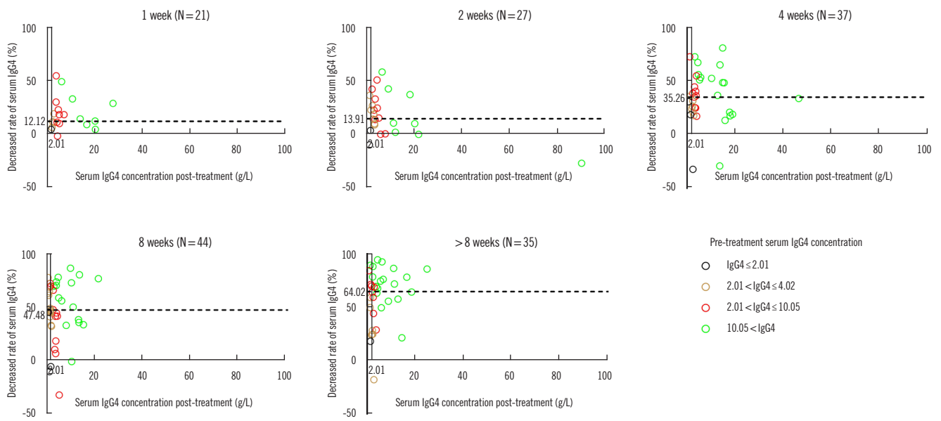
Supplemental Data Fig. S4. Serum IgG4 concentrations post-treatment and decrease rate of serum IgG4 concentration over follow-up, stratified by pre-treatment serum IgG4 concentration. The dashed line parallel to the X-axis represents the median decrease rate of serum IgG4 concentration. The solid line parallel to the Y-axis represents the reference serum IgG4 concentration (2.01 g/L).
