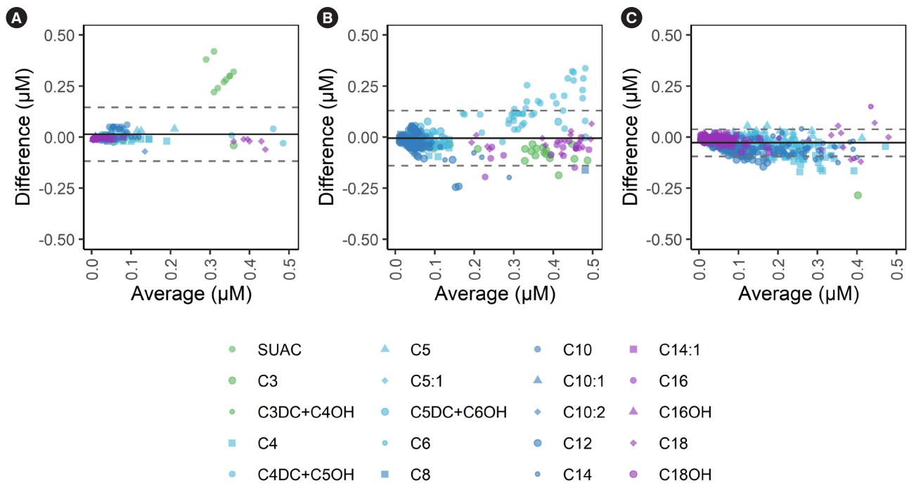
Supplemental Data Fig. S2. Bland–Altman plots with average <math>< 0.5 \mu\text{M}</math> comparing the NeoBase 2 non-derivatized assay results with (A) NSQAP participants using the NeoBase 2 non-derivatized assay for amino acids, SUAC, and acylcarnitines, (B) KEQAS participants regardless of the assay for amino acids and acylcarnitines, and (C) our in-house derivatized assay.
