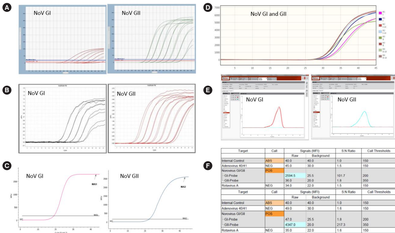
Supplemental Data Fig. S1. Verification of the synthetic norovirus GI and GII RNAs using six commercial norovirus detection kits: (A) AccuPower Norovirus Real-Time RT-PCR Kit (Bioneer), (B) PowerChek Norovirus GI/GII Multiplex Real-Time PCR Kit (Kogene Biotech), (C) Allplex Gastrointestinal Panel Assays (Seegene), (D) BD MAX Enteric Viral Panel (Becton Dickinson), (E) FilmArray Gastrointestinal Panel (BioFire Diagnostics), and (F) Luminex xTAG Gastrointestinal Pathogen Panel (Luminex). Abbreviation: NoV, norovirus.
