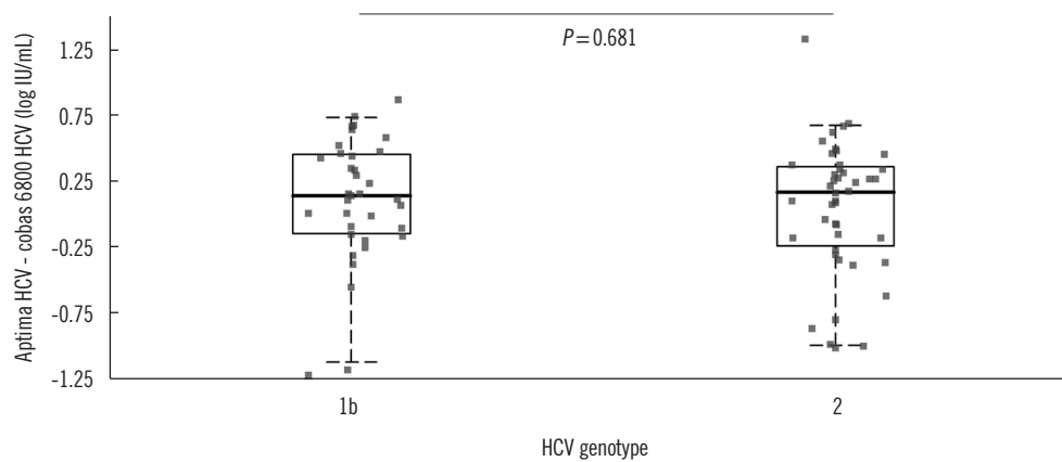
Supplemental Data Figure S1. HCV genotype (genotype 1b, N=35; genotype 2, N=44) and difference in HCV results between the Aptima and cobas 6800 assays.
