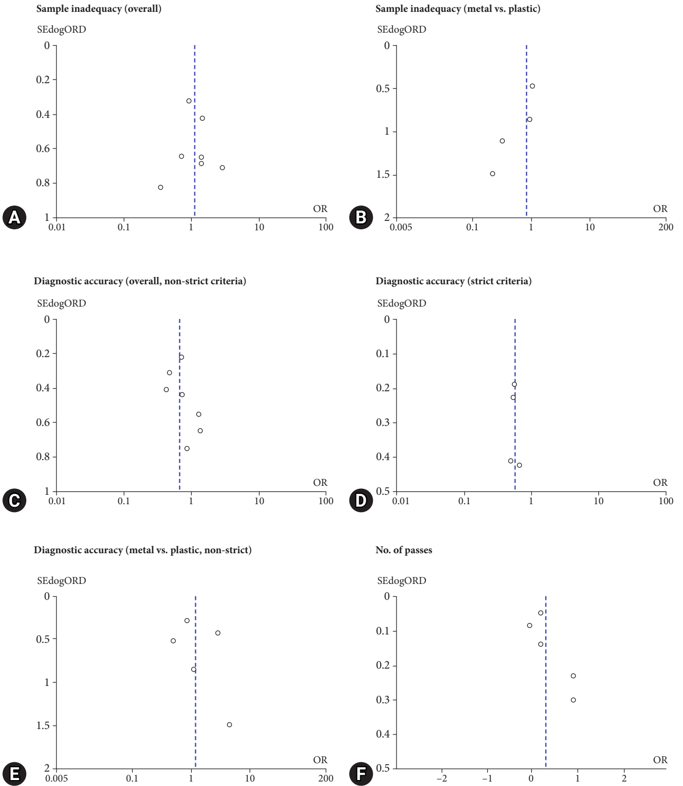
Supplementary Fig. 5. Funnel plot for assessment of publication bias
