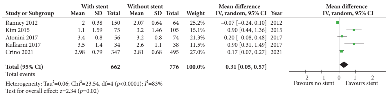
Supplementary Fig. 4. Forest plot comparing the number of passes with EUS-guided pancreatic tissue acquisition with and without biliary stent
