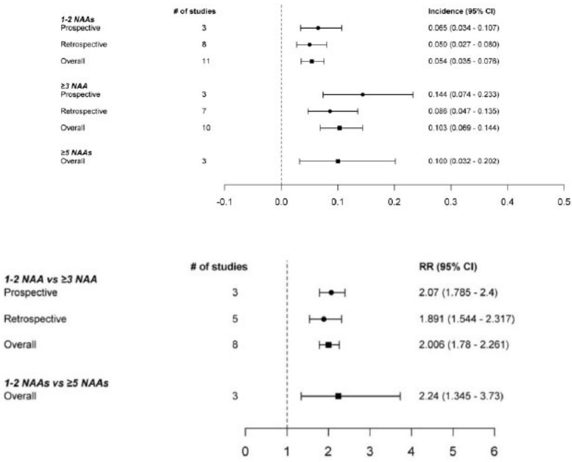
Supplementary Fig. 1. The incidence and relative risk of metachronous colorectal advanced neoplasia in the meta-analysis.
