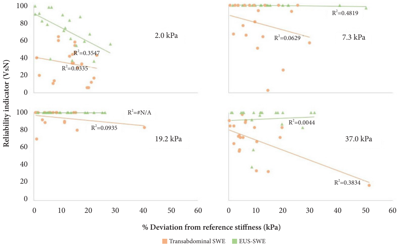
Supplementary Fig. 2. Correlation between the reliability indicator and accuracy of the measurements at varying stiffness values. Scatter-plot analysis of all measurements, plotted as percentage deviations from the reference stiffness values compared with the reliability indicator. All trendlines had R^2 values of <0.5 , indicating a poor correlation between the two variables. For 19.2 kPa, an R^2 value for EUS-SWE was not reported, as all values had a VsN of 100%. VsN, reliability indicator; EUS-SWE, endoscopic ultrasound shear wave elastography.
