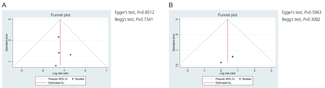
Supplementary Fig. 4. Funnel plots for publication bias of the safety endpoints: (A) rate of nausea plus vomiting; and (B) diarrhea. CI, confidence interval.
