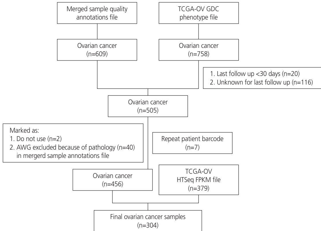
Supplementary Fig. 1. A workflow of the quality control process of TCGA-OV samples. TCGA-OV, The Cancer Genome Atlas-Ovarian Cancer; GDC, genomic data commons, AWG, analysis working group; FPKM, fragments per kilobase of transcript per million.
