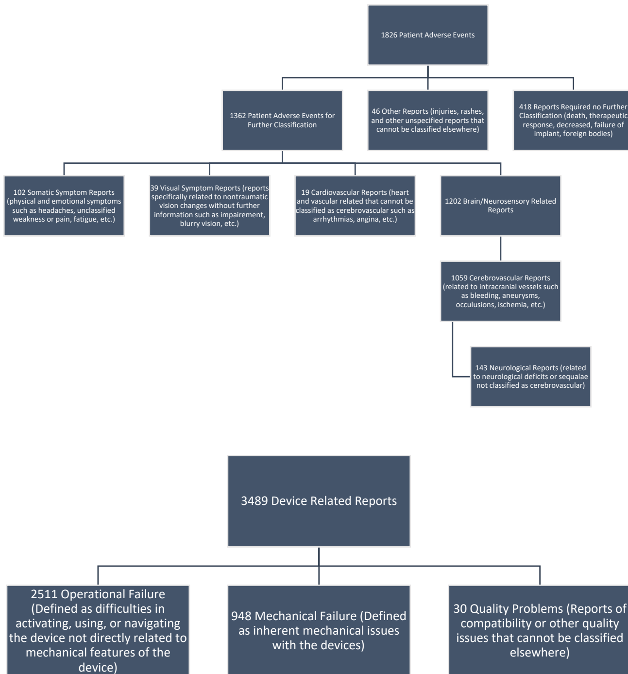
Supplementary Fig. 1. PR event data classification process
