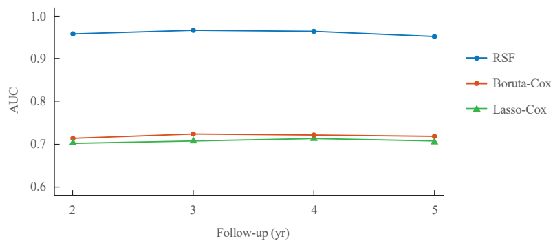
Supplemental Fig. S2. Time-dependent area under the curve (AUC) in the training set. Random survival forest (RSF). Cox proportional hazards regression with Boruta-selected features (Boruta-Cox). Least absolute shrinkage and selection operator (LASSO)-penalized Cox proportional hazards regression (LASSO-Cox).
