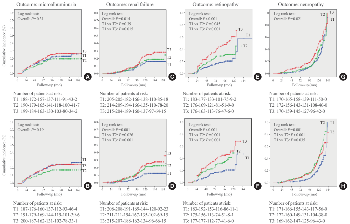
Supplemental Fig. S4. Kaplan-Meier curves of cumulative incidence of microvascular outcomes in patients grouped according to tertiles of 1st-year hemoglobin glycation index variability (top panels A, C, E, and G) and according to tertiles of 1st-year glycated hemoglobin variability (bottom panels B, D, F, and H). T1 is the lower tertile subgroup (blue line), T2 the middle tertile subgroup (green line), and T3 is the upper tertile subgroup (red line).
