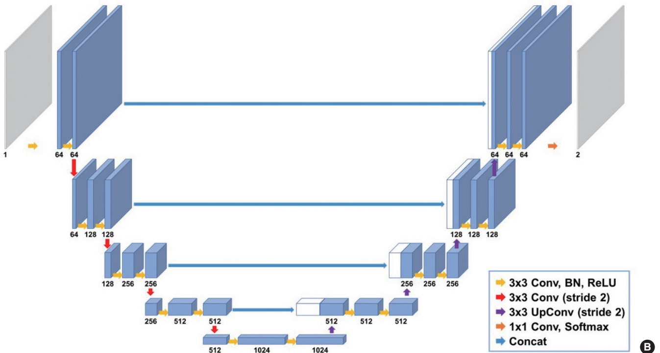
Supplemental Fig. S2. (A) Proposed semi-supervised learning model for the lumbar segmentation method. (B) The architecture of the segmentation network. L_{CE} , cross-entropy loss; Y , predicted segmentation map; L_{MS CNN} , Mumford-Shah loss; Conv, convolution; BN, batch norm; ReLU, rectified linear unit.
