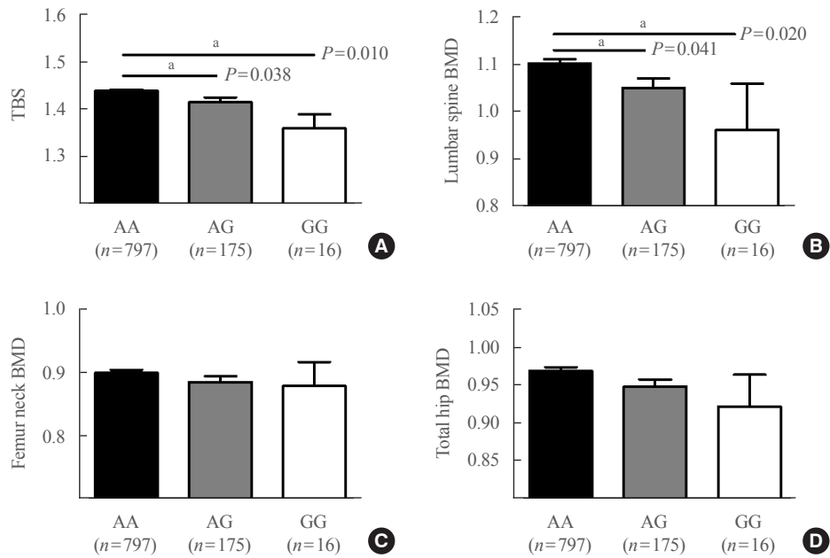
Supplemental Fig. S1. (A) Trabecular bone score (TBS), (B) lumbar spine, (C) femur neck, and (D) total hip bone mineral density (BMD) according to rs1815994 variants in men from the discovery cohort. a P < 0.05 from analysis of variance.
