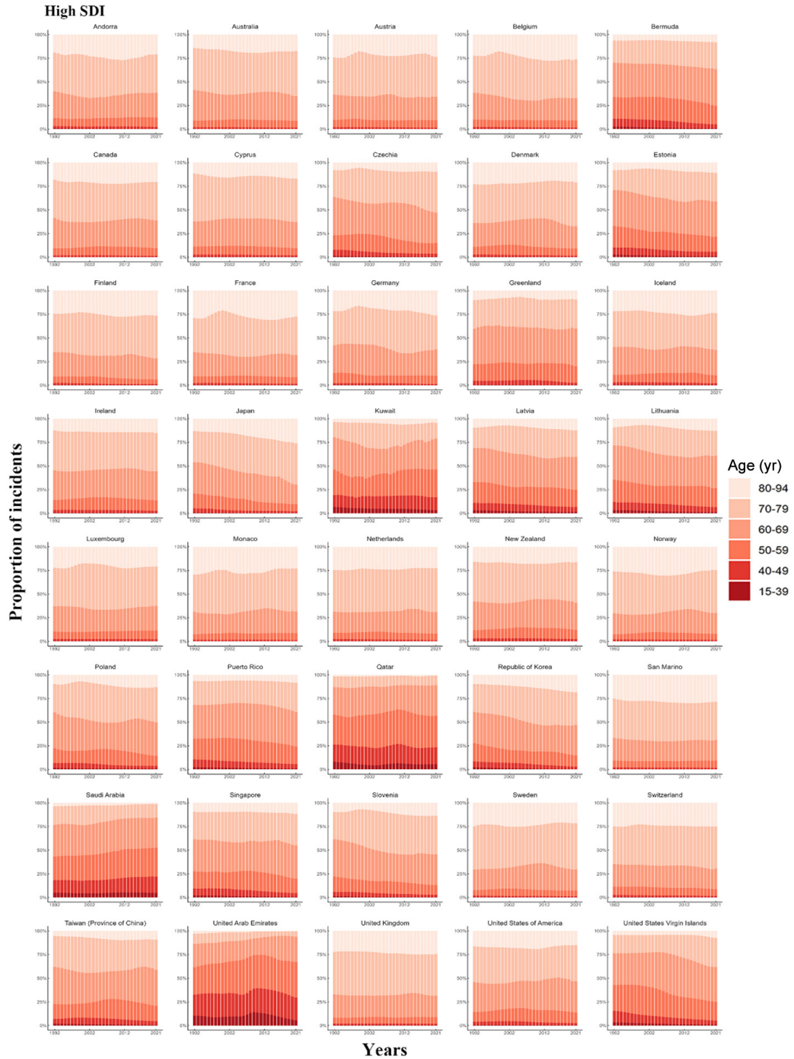
Supplementary Fig. 6. Age distribution of incidences from type 2 diabetes mellitus related chronic kidney disease in high sociodemographic index (SDI) countries, 1992–2021.
