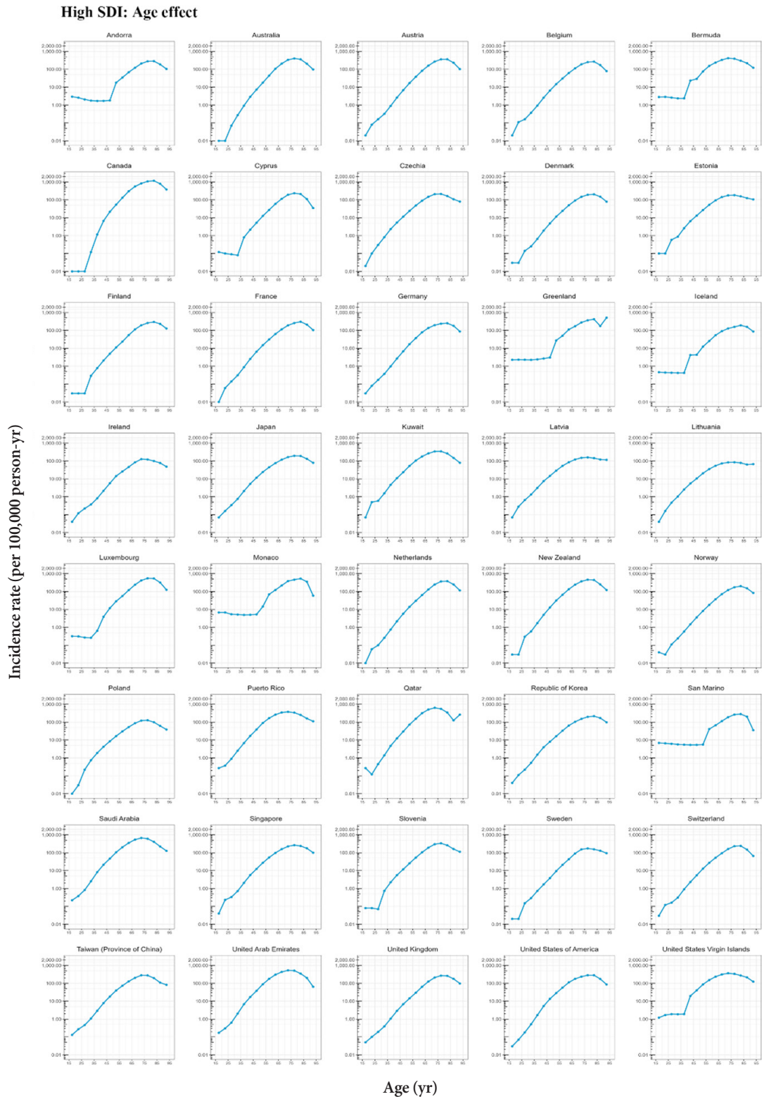
Supplementary Fig. 11. Age effects on type 2 diabetes mellitus related chronic kidney disease incidence rate in high sociodemographic index (SDI) countries.
