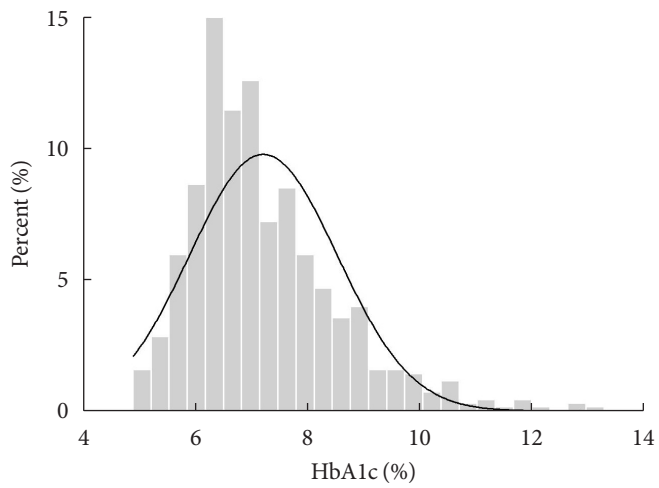
Supplementary Fig. 1. A histogram showing distribution of baseline glycosylated hemoglobin (HbA1c) levels.
