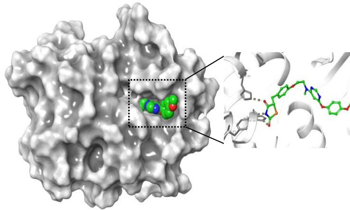
Supplementary Fig. 1. X-ray crystallographic structure of lobeglitazone (green) bound to the active site of peroxisome proliferator-activated receptor \gamma .
