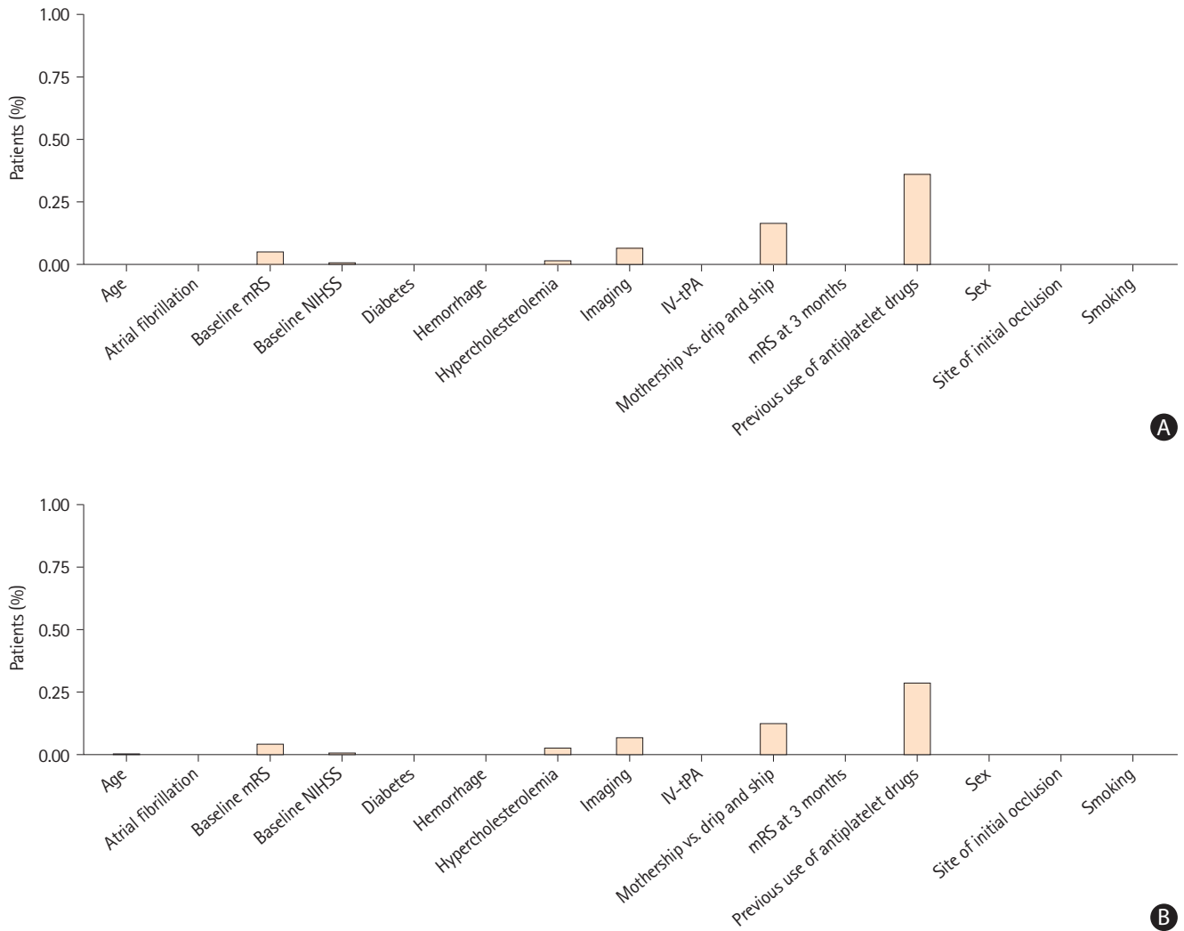
Supplementary Figure 1. Proportion of missing data per variable. (A) Missing variables after PSM. (B) Missing variables before PSM. PSM, propensity score matching; mRS, modified Rankin Scale; NIHSS, National Institutes of Health Stroke Scale; IV-tPA, intravenous tissue plasminogen activator.
