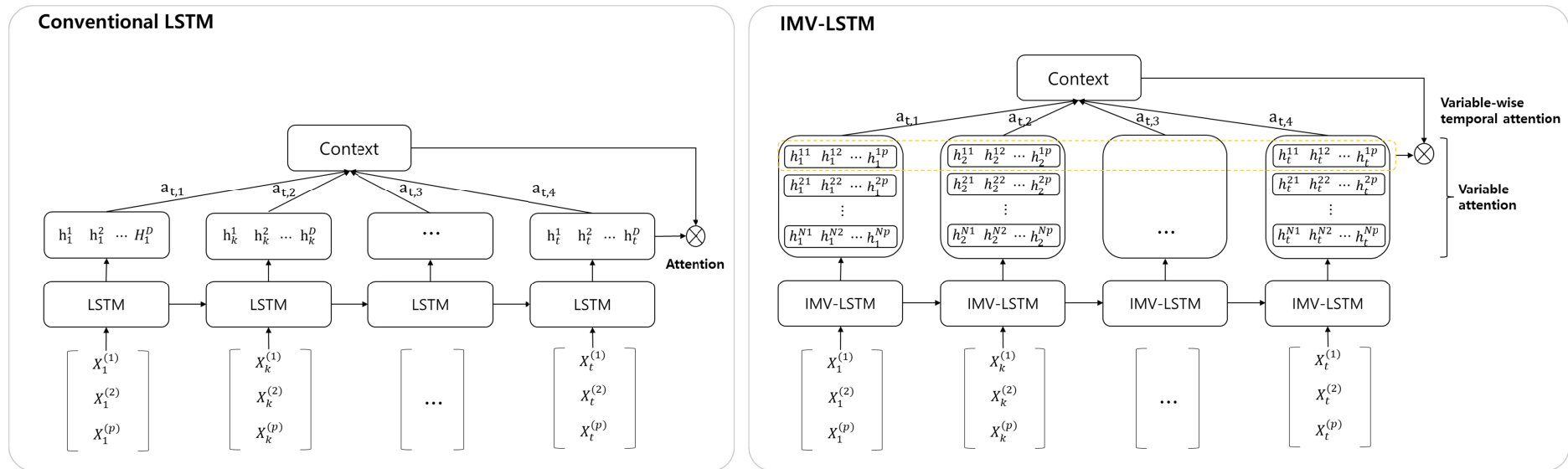
Figure S1. Model architecture of interpretable multi-variable long short-term memory (IMV LSTM). X: input, p: number of features, t: time step, h: hidden state, a: attention score.
