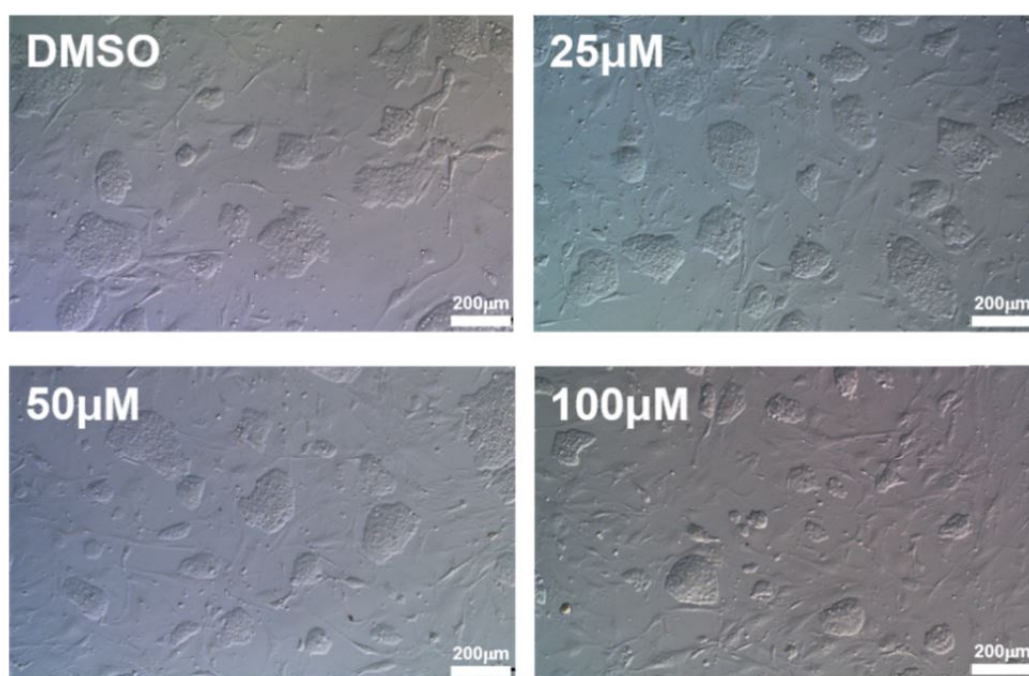
Fig. S1. Effect of Dnmt inhibitor 5-AzaC on the proliferation of embryonic stem cells. Treatment of various concentrations of 5-AzaC did not affect the self-renewal abilities of ESCs. Scale bars: 200 \mu m.
