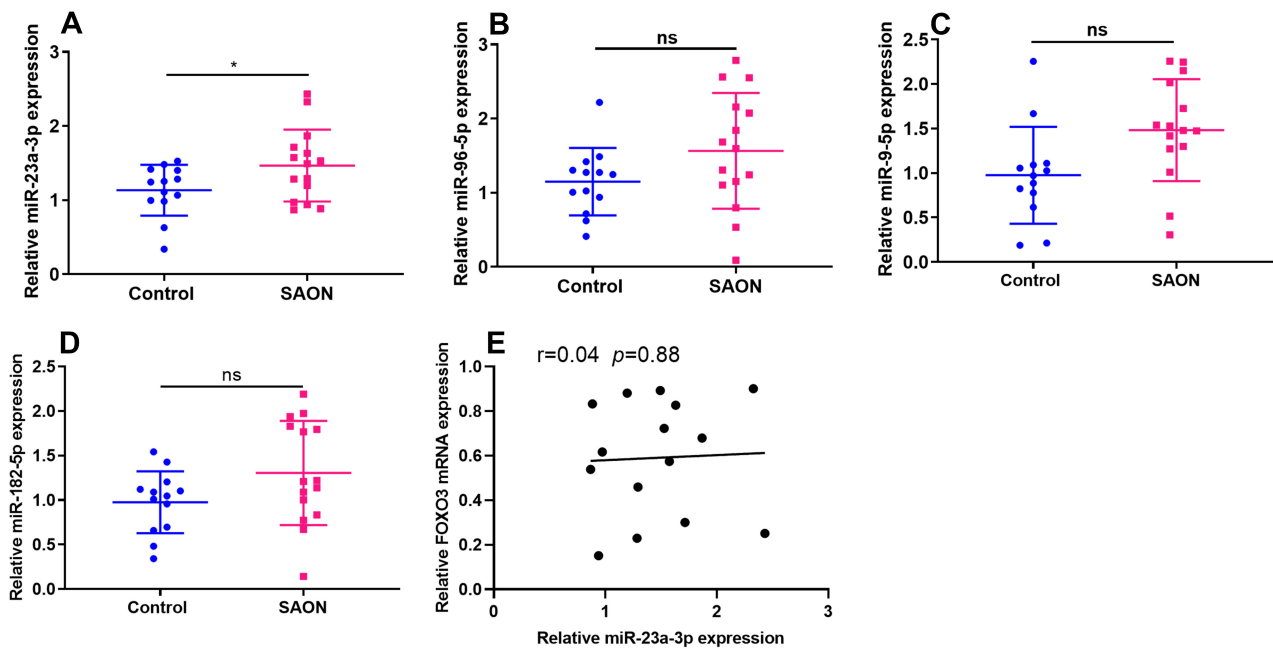
Fig. S1. The expression of miR-23a-3p, miR-96-5p, miR-9-5p and miR-182-5p in SAON patients and control individuals. (A) qRT-PCR was used to detect the expression of miR-23a-3p in the samples of SAON patients and control individuals. (B) qRT-PCR was used to detect the expression of miR-96-5p in the samples of SAON patients and control individuals. (C) qRT-PCR was used to detect the expression of miR-9-5p in the samples of SAON patients and control individuals. (D) qRT-PCR was used to detect the expression of miR-182-5p in the samples of SAON patients and control individuals. (E) Correlations between the expression of miR-23a-3p and FOXO3 in the samples of SAON patients. * p < 0.05 .
