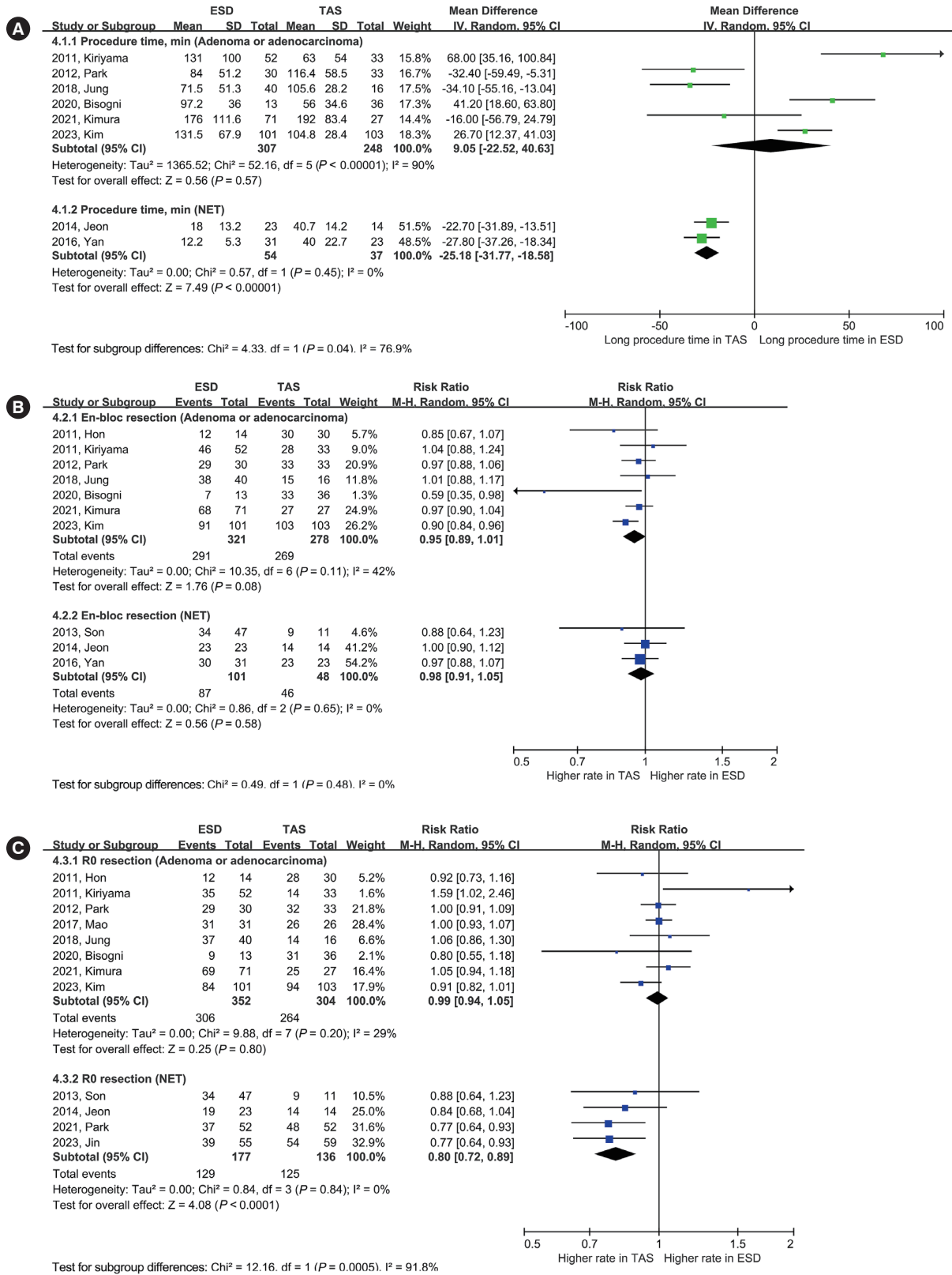
Supplementary Fig. 2. Forest plots for short-term clinical outcomes between endoscopic submucosal dissection and transanal surgery. (A) Procedure time, (B) en bloc resection, and (C) R0 resection. ESD, endoscopic submucosal dissection; TAS, transanal surgery; SD, standard deviation; IV, inverse variance; CI, confidence interval; NET, neuroendocrine tumor; M-H, Mantel-Haenszel.
