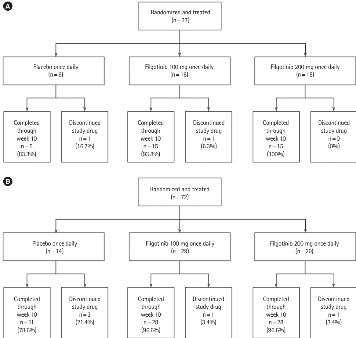
Supplementary Fig. 2. Disposition of Japanese patients in induction study A (biologic-naïve patients) (A) and induction study B (biologic-experienced patients) (B).
