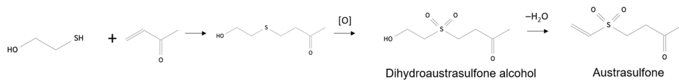
Supplementary Fig. 1. Synthesis of active compound. Synthetic route for dihydroaustrasulfone alcohol and austrasulfone.
