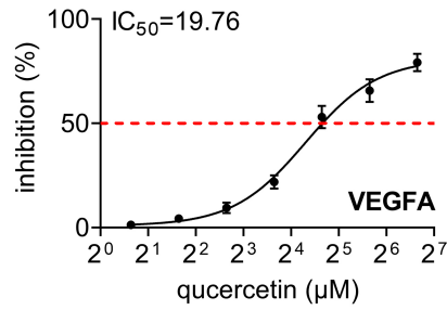
Supplementary Fig. 1. Inhibition of kinase activity by quercetin. Z'-LYTE kinase inhibition assay to inhibitory effect of quercetin to top 5 proteins (AKT, TP53, TNF, IL6, and VEGFA). The half inhibition rate ( \text{IC}_{50} ) was also calculated. The \text{IC}_{50} values of quercetin on AKT, TP53, TNF, IL6, and VEGFA were 2.288 \mu\text{M} , 4.037 \mu\text{M} , 8.753 \mu\text{M} , 14.31 \mu\text{M} , and 19.76 \mu\text{M} , respectively.
