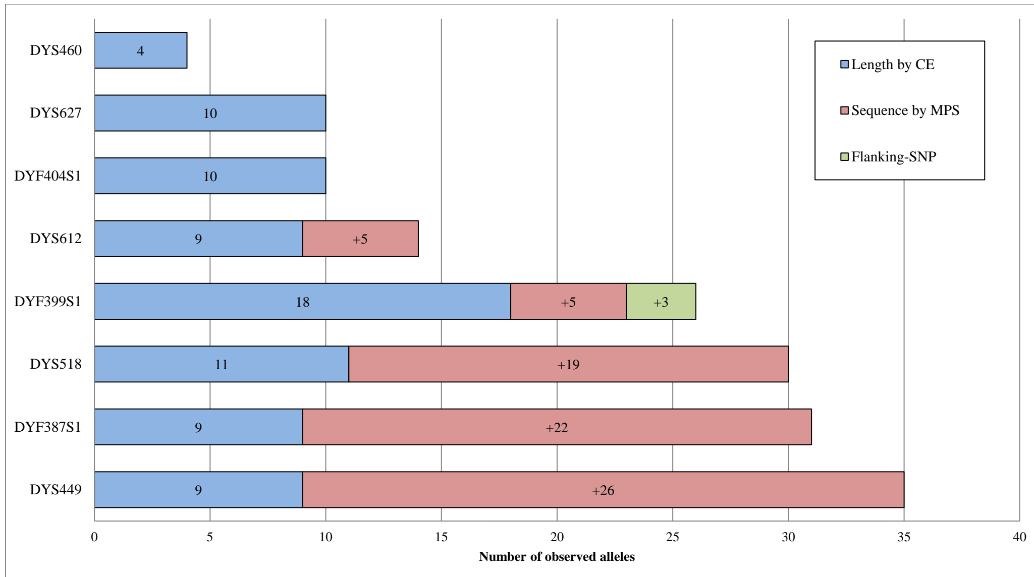
Supplementary Fig. 6. Comparison of the number of observed alleles by CE and MPS analysis of additional 8 Y-chromosomal STRs in Koreans (n = 105). This figure is shown for the markers except as reported by Kwon et al. 17
