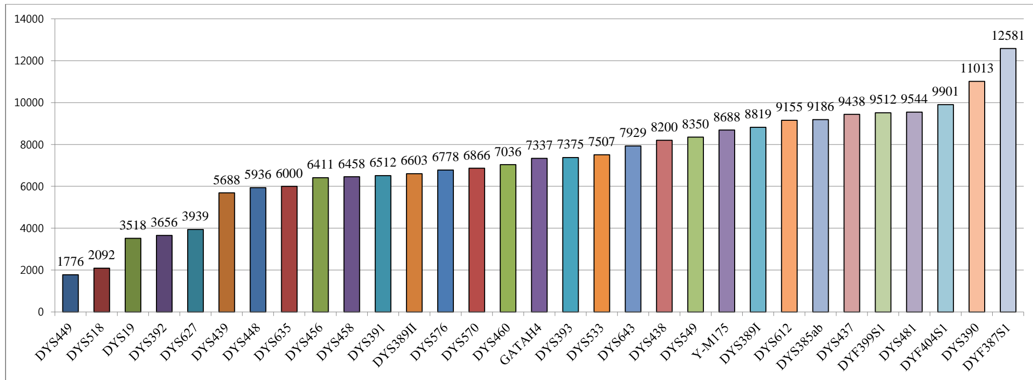
Supplementary Fig. 2. Average DoC for the 32 Y-chromosomal markers used in this study for all 220 male DNA samples of 1ng/ \mu L. Loci were sorted in ascending order of marker coverage. The numbers on each bar represent the average DoC of each marker.
