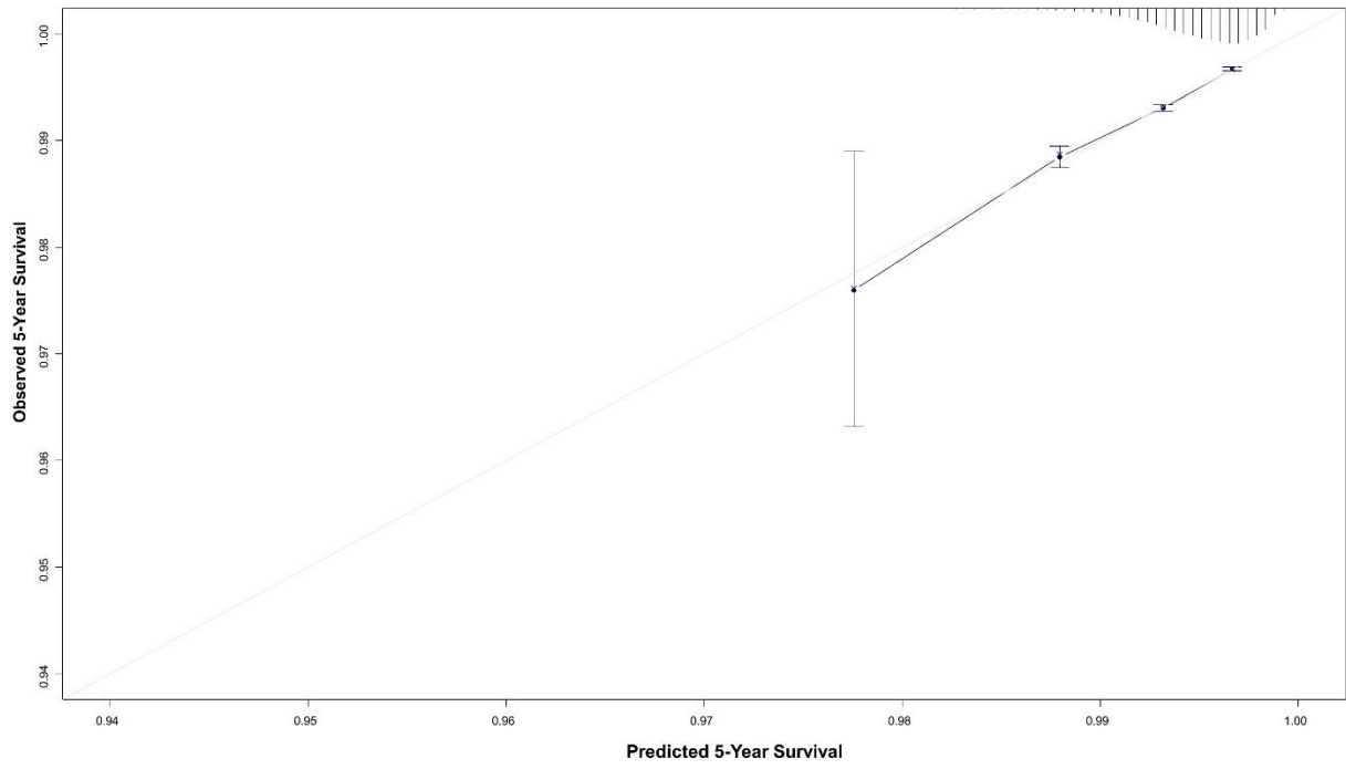
S7 Fig. Calibration plot of the breast cancer risk-prediction model in postmenopausal women.
