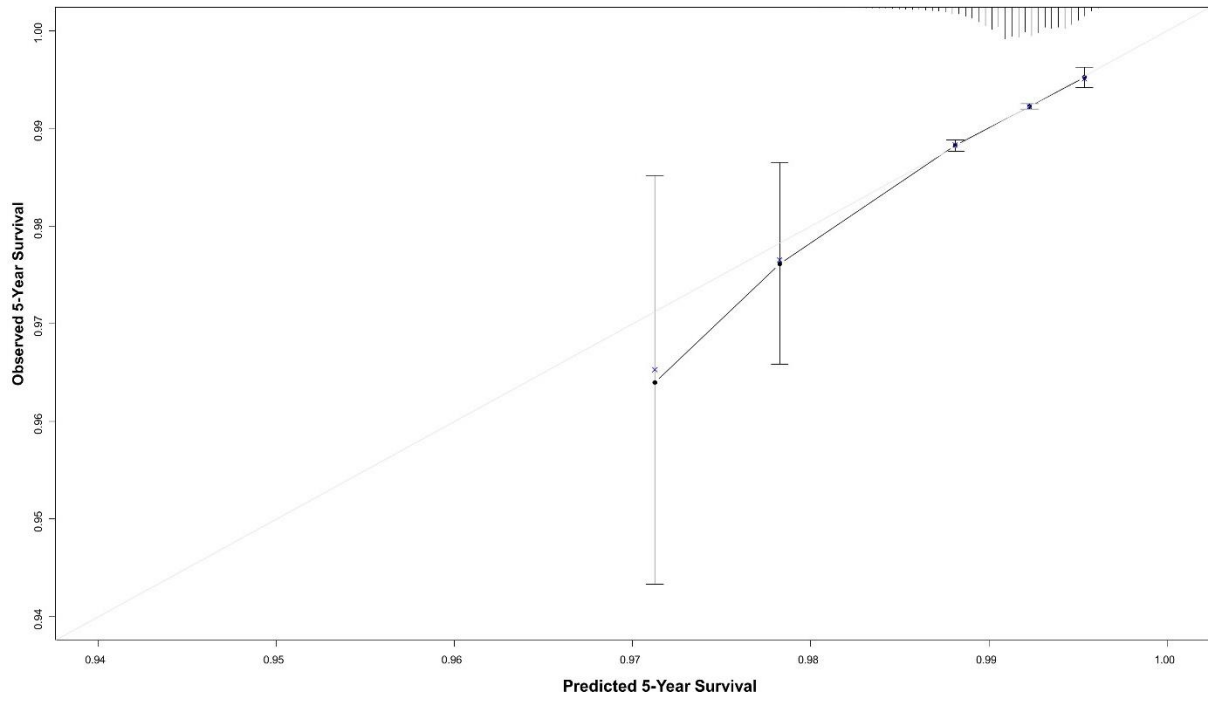
S6 Fig. Calibration plot of the breast cancer risk-prediction model in premenopausal women.
