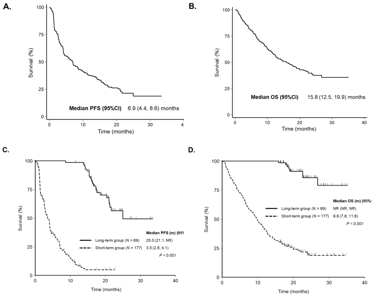
S3 Fig. Survival outcomes. Progression-free survival (PFS) (A) and overall survival (OS) (B) of the overall population. PFS (C) and OS (D) based on the atezolizumab plus bevacizumab treatment duration (short-term group [ < 1 year] vs. long-term group [ \geq 1 year]). CI, confidence interval; NR, not reached.
