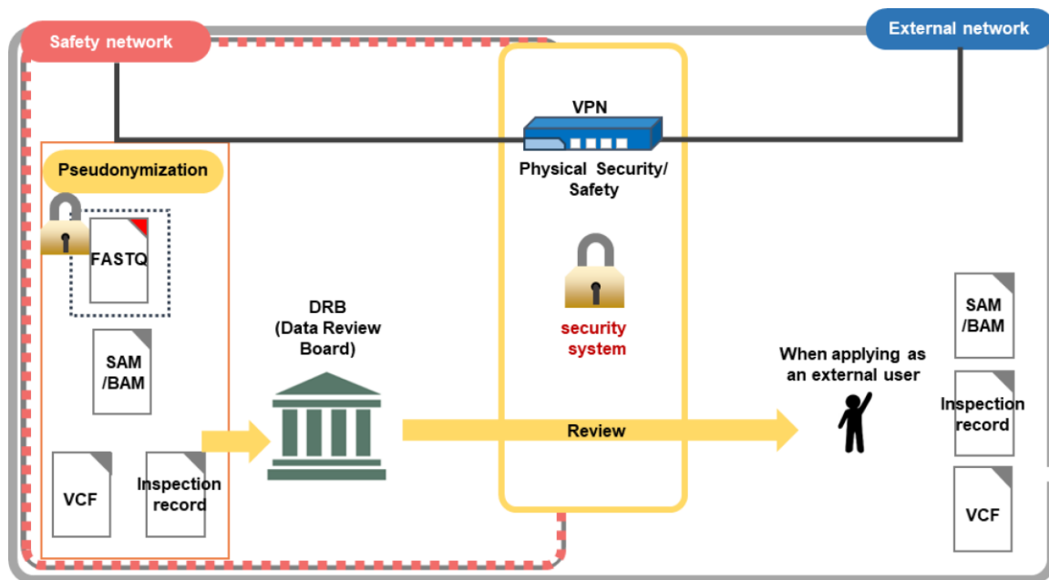
S15 Fig. Network safety measures for utilizing genomic data. BAM/SAM and FASTQ files contain detailed sequence information, and during secondary processing, there may be data that requires pseudonymization. In the case of FASTQ files, it is advisable to export only the analysis results in the form of VCF files after internal analysis. Pseudonymized VCF files are considered suitable for external export.
