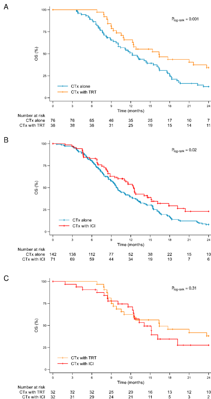
S8 Fig. Kaplan-Meier curves of overall survival in the propensity-score matched cohorts. Matched cohorts were constructed using 2:1 (chemotherapy/TRT), 2:1 (chemotherapy/ICI), and 1:1 (TRT/ICI) ratios. CTx, chemotherapy; ICI, immune checkpoint inhibitor; OS, overall survival; TRT, thoracic radiotherapy.
