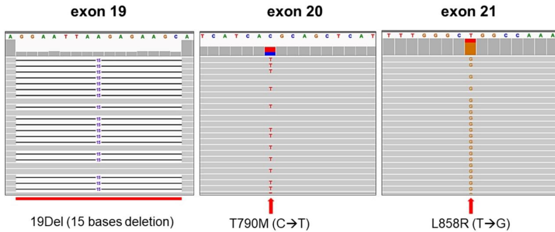
S6 Fig. The result from the detection of epidermal growth factor receptor ( EGFR ) mutations based on blocker displacement amplification amplicon Nanopore sequencing was visualized by the IGV tool. The 19Del (15 bases deletion), T790M, and L858R mutations were found in exon 19, 20, and 21, respectively.
