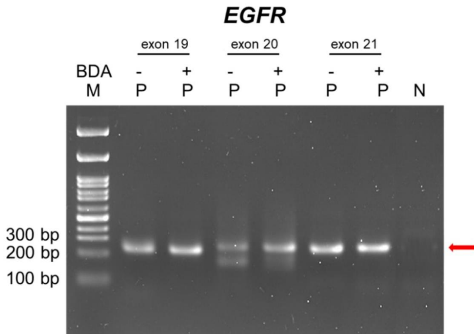
S4 Fig. The cancer cell lines (H1650 and H1975) were used for templates to amplify epidermal growth factor receptor ( EGFR ) in each exon by with and without blockers in the polymerase chain reaction. All amplicons were tagged with the barcode and investigated by gel electrophoresis. The red pointer representing amplicon products were 240 bp, 248 bp, and 241 bp of exon 19, 20, and 21, respectively. BDA, blocker displacement amplification.
