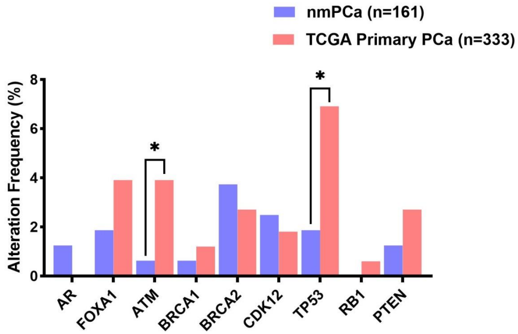
S1 Fig. The comparison of the alteration frequencies between the non-metastatic prostate cancer (nmPCa) patients in our cohort and the primary PCa patients in The Cancer Genome Atlas (TCGA) cohort.
