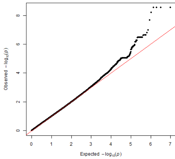
S1 Fig. Q-Q plot. The observed p-value (y-axis) was compared with the expected raw p-value (x-axis, under null distribution).
