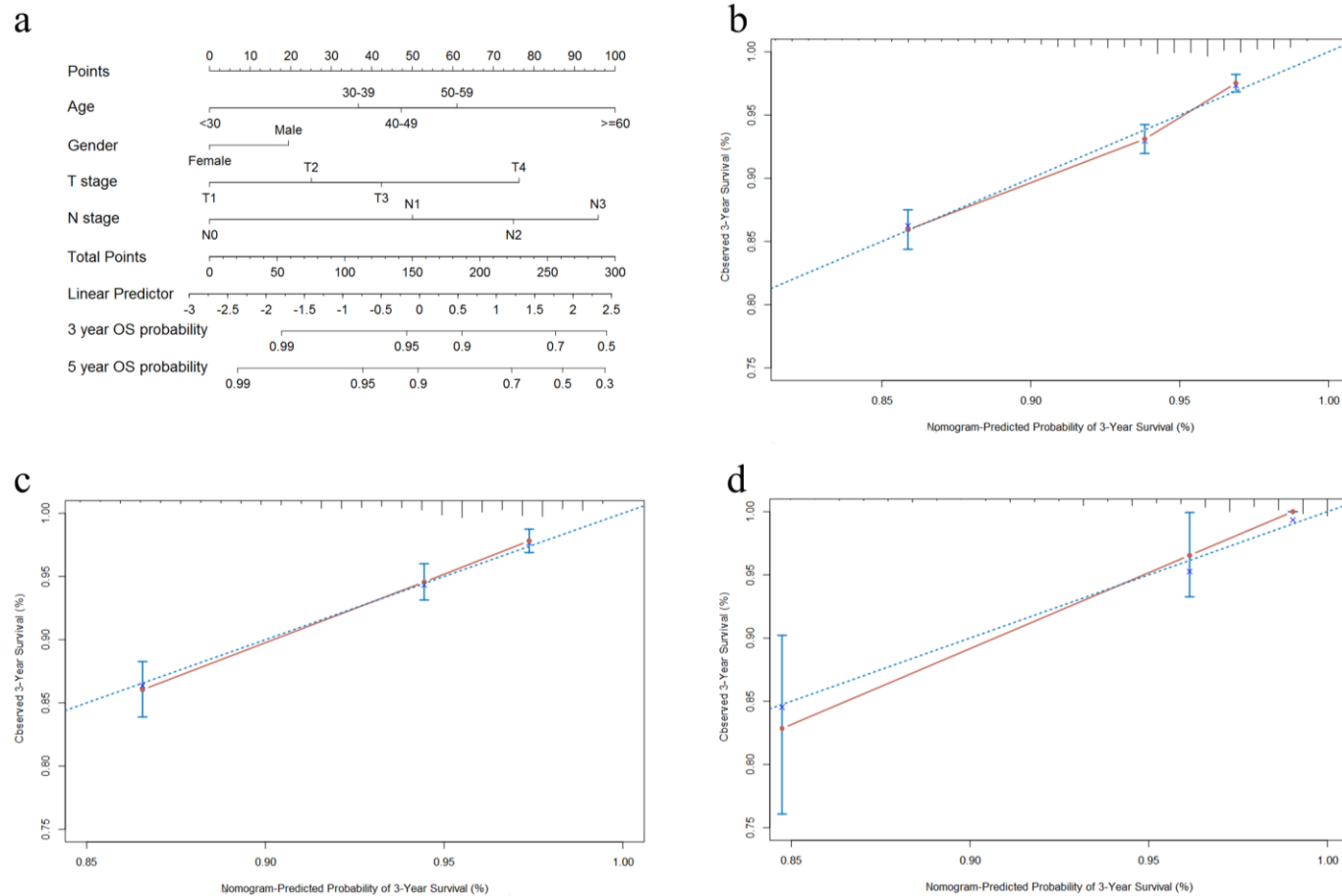
S2 Fig. (A) Nomogram for 3- and 5-year overall survival (OS) in nasopharyngeal carcinoma patients. Calibration curve of nomogram for predicting 3-year local relapse-free survival (LRFS) for the training cohort (B), internal validation cohort (C), and external validation cohort (D). Actual LRFS plotted on the y-axis; nomogram predicted probability of LRFS plotted on the x-axis.
