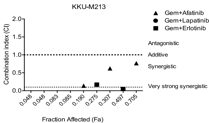
S4 Fig. Combination index value (CI) of gemcitabine and ErbB inhibitors treatment in HuCCA-1 (A) and KKU-M213 (B).
