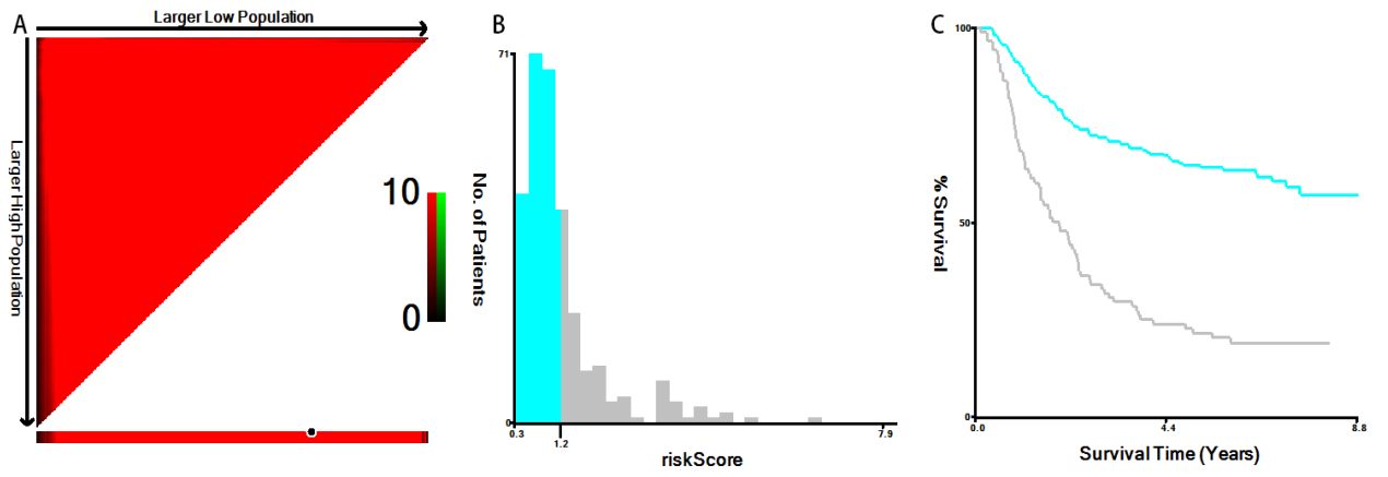
S4 Fig. The optimal cutoff value of risk score was determined by X-tile software. The optimal cutoff value highlighted by the black dot in part A is shown on a histogram of the entire cohort (B) and a K-M plot (C).
