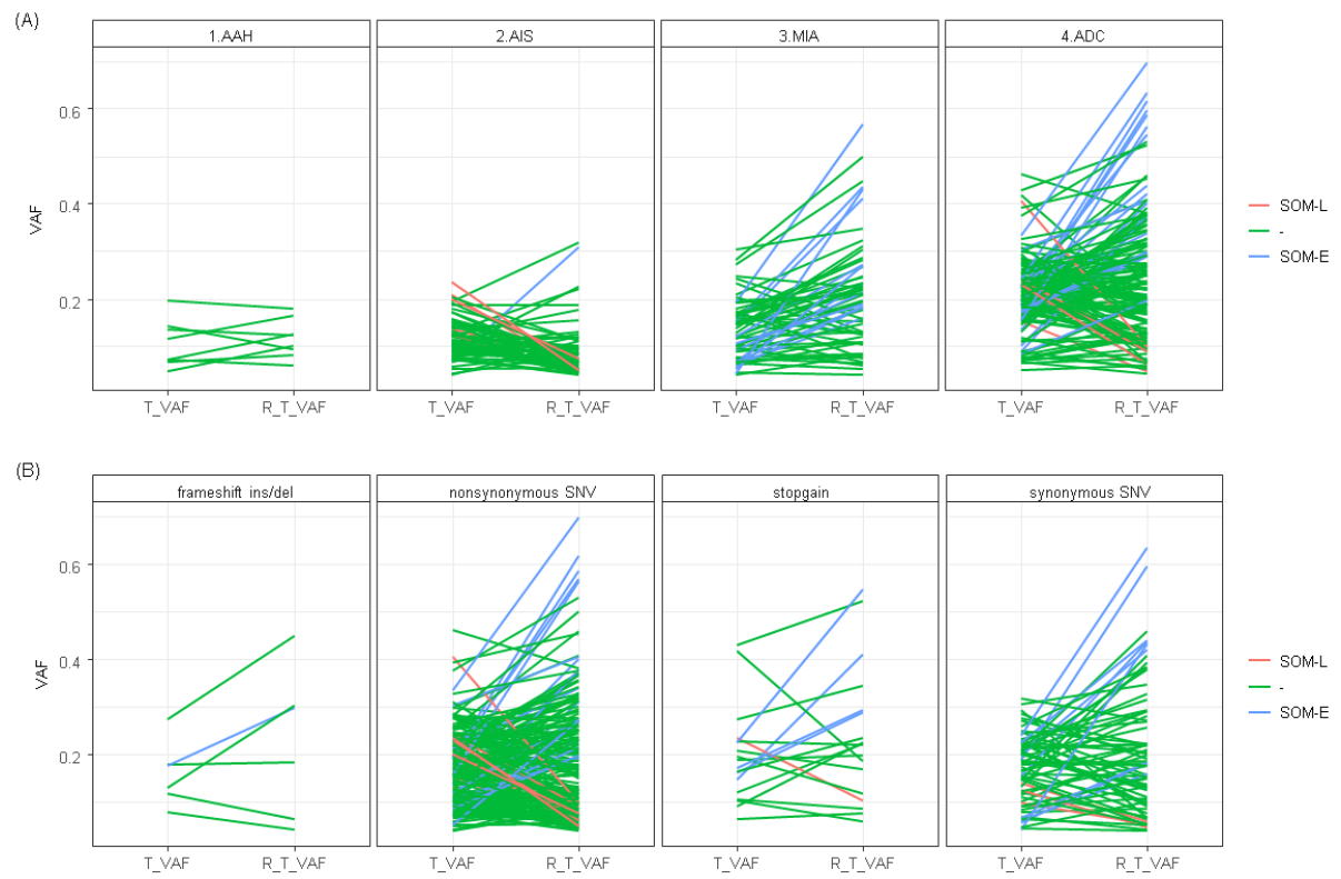
S9 Fig. Relationship between whole exome sequencing (WES) variant allele frequency (VAF) and RNA VAF across lesion types (A) and variant annotations (B).
