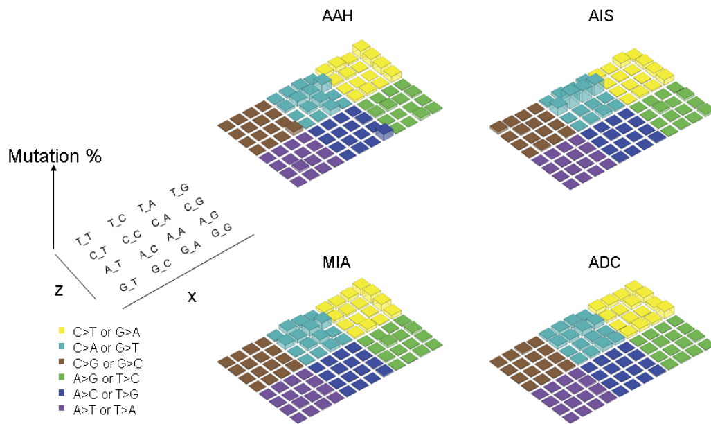
S7 Fig. Lego plots showing the average frequency of base substitutions within specific trinucleotide mutational contexts. AAH, atypical adenomatous hyperplasia; ADC, adenocarcinoma; AIS, adenocarcinoma in situ ; MIA, minimally invasive adenocarcinoma.
