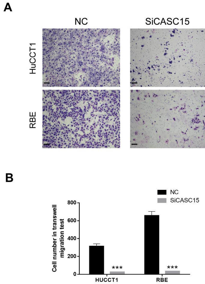
S1 Fig. Knockdown of cancer-associated susceptibility 15 (CASC15) decreased the migration of intrahepatic cholangiocarcinoma cells. (A, B) Transwell migration experiment of siCASC15 and control group and quantitative results. Scale bars=100 \mu m. *** p < 0.001 .
