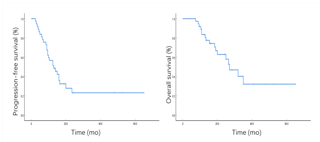
S2 Fig. Kaplan-Meier estimates of progression-free survival and overall survival of the entire cohort.
