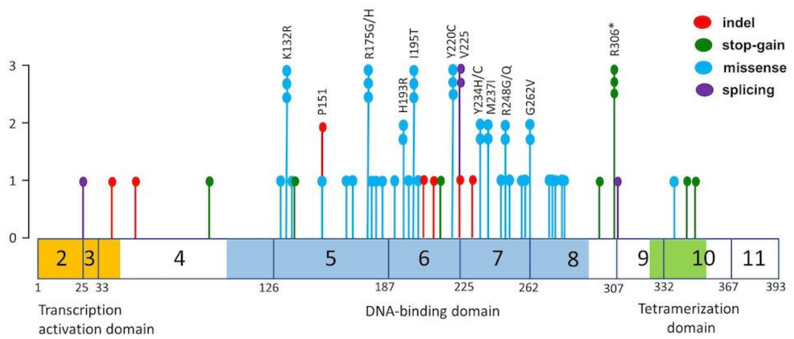
S5 Fig. The details of the TP53 gene mutation in this study is shown in graphic chart. TP53 mutations were significantly enriched in DNA-binding domain.
